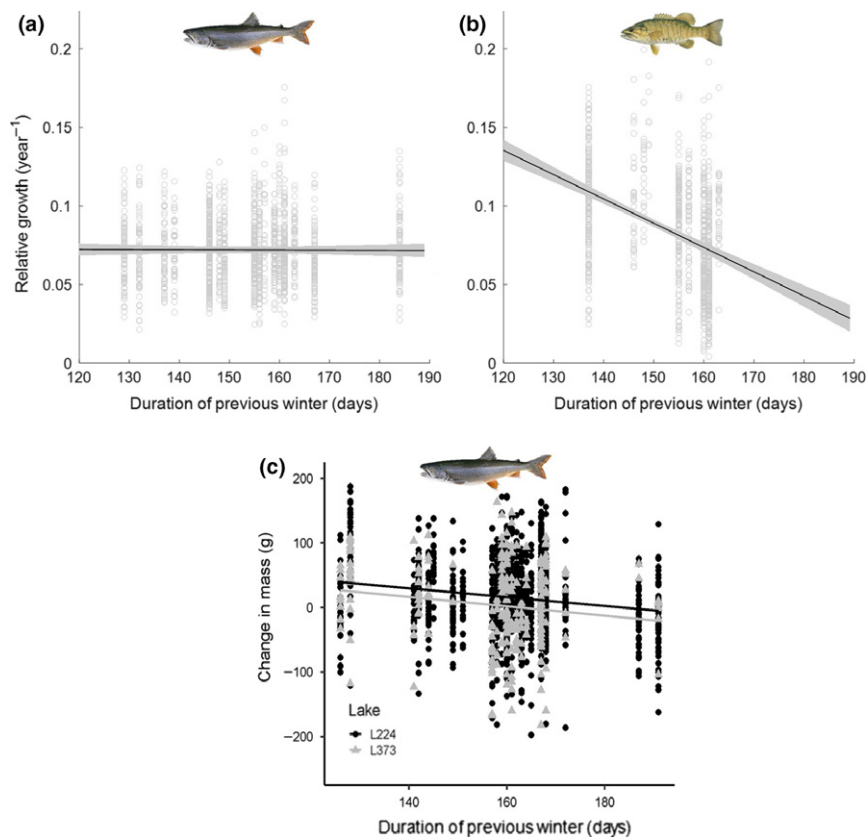
Figure 4 Individual growth of lake trout (a and c) and smallmouth bass (b) in response to inter-annual changes in winter duration (days). Data from Lake Opeongo, Ontario, Canada (a, b; cm per year relative to maximum length) demonstrate that lake trout are more tolerant to winter duration than smallmouth bass. In smaller lakes lacking an offshore forage fish (Experimental Lakes Area Lake 224 and Lake 373), like our study lake described in Case Study #1 (Box 1), however, individual lake trout mass (g) declines in years with the longest winters (c). See Supporting Information S2 for details on growth calculation and data analysis.
