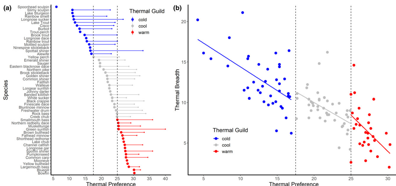
Figure 2 Thermal preferences and thermal niche breadth for Canadian freshwater fishes belonging to three thermal guilds: cold-water, cool-water, and warm-water. (a) The continuous distribution of thermal preference (large left point) and upper thermal limit (small right point) for 54 of the most common Canadian freshwater fishes. (b) The relationship between thermal preference and thermal breadth (upper thermal limit – thermal preference) for 114 species across the three thermal guilds is negative. These data support thermal performance trade-offs in freshwater fishes. Increased performance at cold temperatures should trade-off with reduced performance at warm temperatures (a) and increased performance at warm temperatures should trade-off with reduced thermal breadth (b). Thermal preference is defined as the temperature that the fish gravitate towards when provided with a broad range of temperatures. Upper thermal limit is the temperature at which 50% mortality occurs in a population. Data for both panels are from Hasnain et al. (2018).
