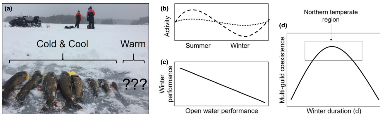
Figure 1 (a) Northern temperate freshwater fishes vary widely in their responses to winter. Those that are better adapted for winter activity are easily captured during winter sampling operations and tend to have colder thermal preferences (a). Other species can be more challenging to capture under ice cover and tend to have warmer thermal preferences (e.g. bass and other sunfishes; a). Being ectotherms, all fishes should be actively foraging during warmer, brighter open water periods, and have reduced activity rates during winter (b). Fishes with colder thermal preferences (short dash), however, are expected to have a higher capacity for winter activity than species with warmer thermal preferences (long dash; b). Optimal performance under a particular set of conditions implies reduced performance under other conditions and sets up a variety of possible trade-offs (Angert et al. 2009; Kingsolver 2009). For example, a high capacity for activity during warm, bright, open water months is expected to trade-off with a reduced capacity for activity during cold, dark winters (c). Seasonal variation broadly and winter periods specifically could therefore favour different species at different times and promote coexistence of species belonging to multiple thermal guilds (d). In northern temperate lakes, winters are likely long enough to support cold-adapted species but not too long so as to exclude warm-adapted species, making this winter-mediated species coexistence particularly likely (d).
