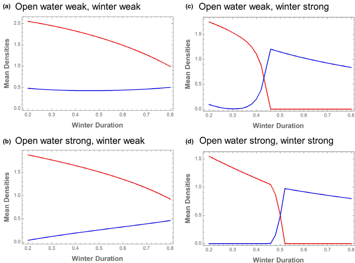
Figure 6 Mean densities of two competing species, one adapted to open water (red) and one to winter (blue) across a gradient of changing winter duration. Four cases were considered, where interspecific competition is either weak or strong in each season. Weak refers to a case where the two species coexist in a given season and strong refers to competitive exclusion in a given season by the species that is best adapted to that season (see Box 3 for detail).
