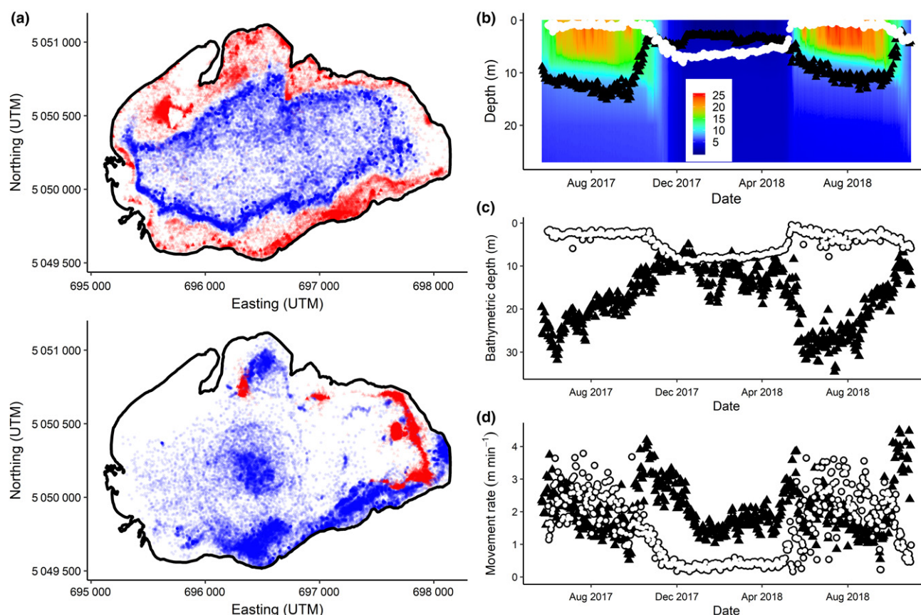
Figure 3 Acoustic telemetry data for lake trout (blue locations and black triangles) and smallmouth bass (red locations and white circles) from Lake of the Two Rivers (Ontario, Canada). (a) Spatial locations of fish in summer (top plot; July and August) and winter (bottom plot; January and February). (b) Mean daily depth (m) of fish within the water column overlaid over the thermal profile (°C) of the lake across the time series. (c) Mean daily bathymetric depth (m) (i.e. depth of water over which fish was positioned). (d) Mean daily activity rates (m min -1 ). For details on the acoustic telemetry data and analyses, see Supporting Information S1.
